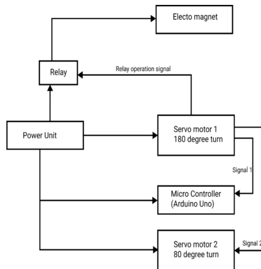
Fig. 7 System operation block diagram
