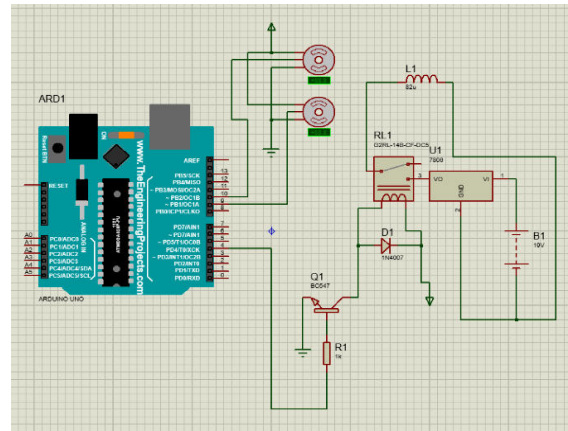
Fig. 9 Circuit diagram
