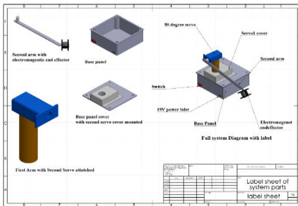
Fig. 5 System parts label
