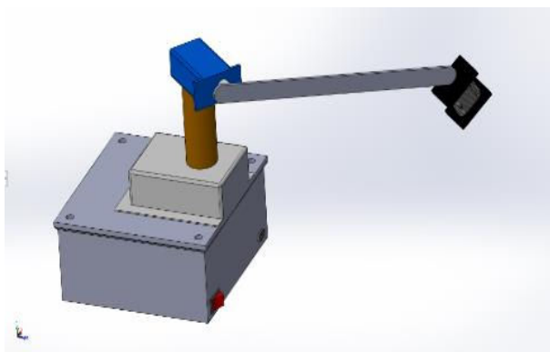
Fig. 6 System 3D model
